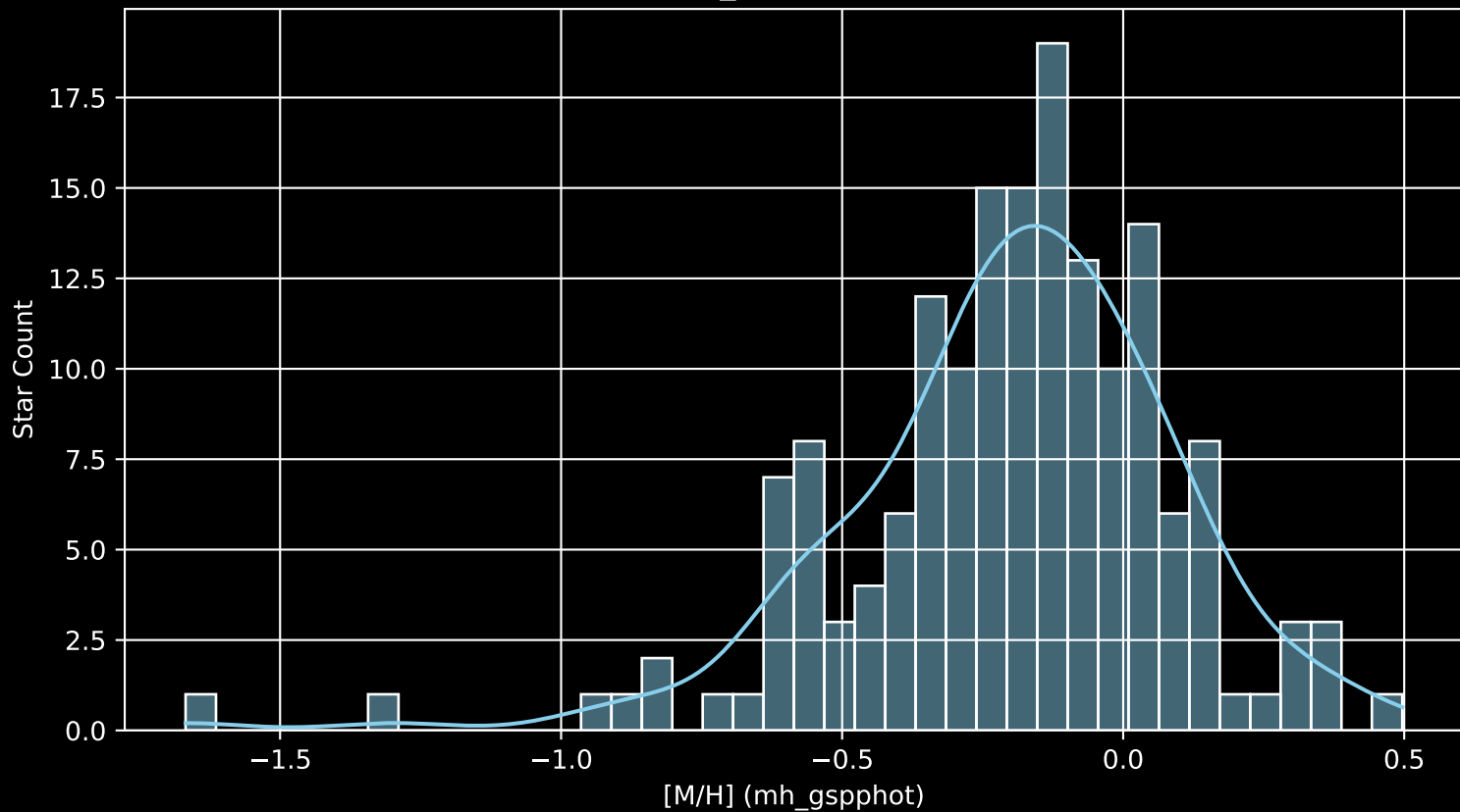
APOGEE DR17 Field: [223+27_MGA [M/H] (mh_gspphot) (n= 167)
