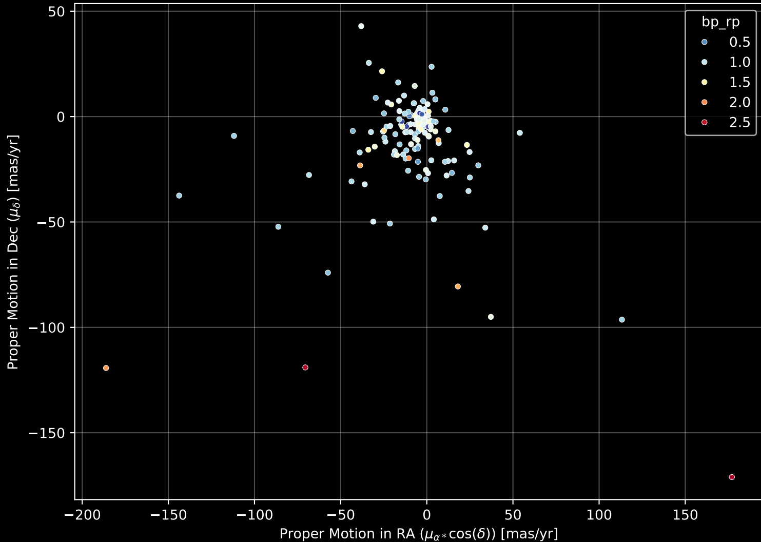
APOGEE DR17 Field: [223+27_MGA] Proper Motion Diagram (n= 167)
