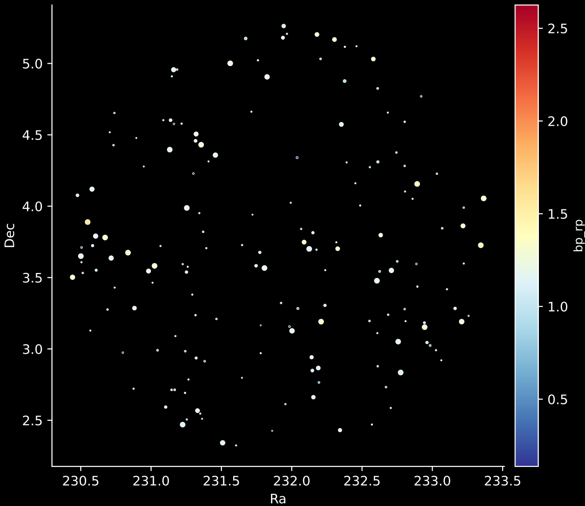
APOGEE DR17 Field: [223+27_MGA] Stars: 167
