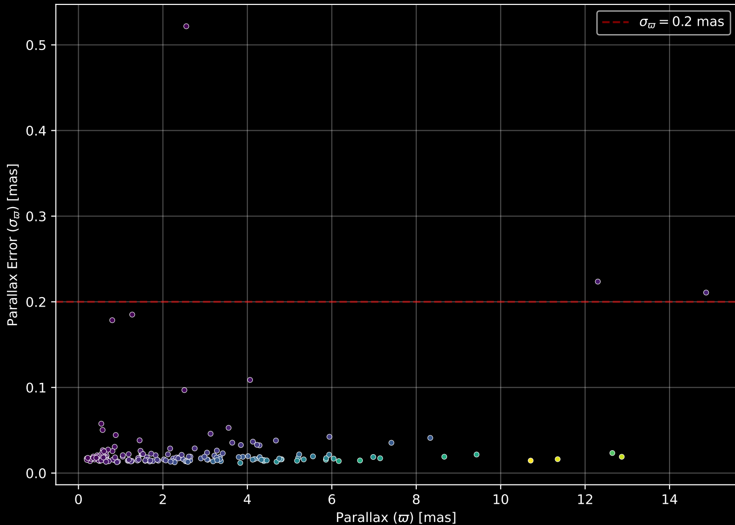
APOGEE DR17 Field: [223+27_MGA] Parallax Quality (n= 167)
