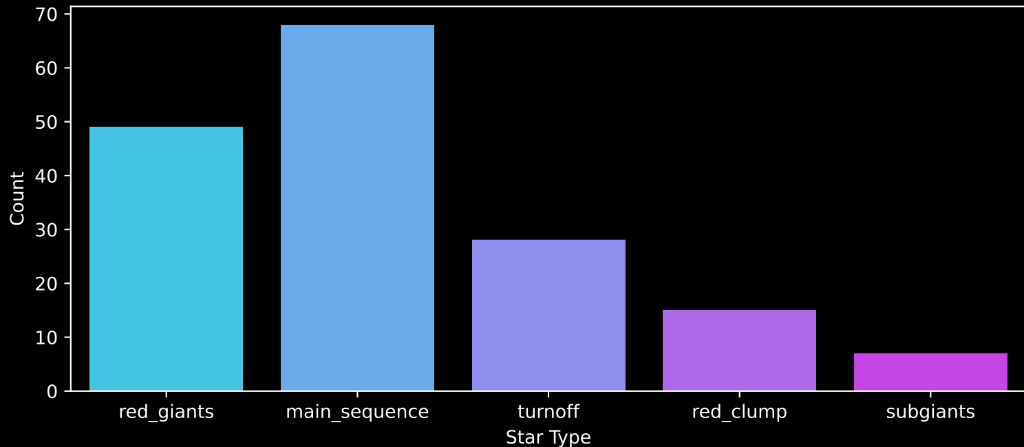
APOGEE DR17 Field: [223+27_MGA] Count plot of Star Type
