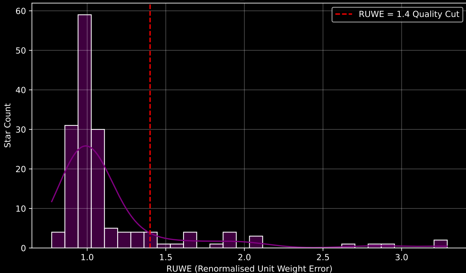
GAPOGEE DR17 Field [223+27_MGA] RUWE Distribution (n= 160)
