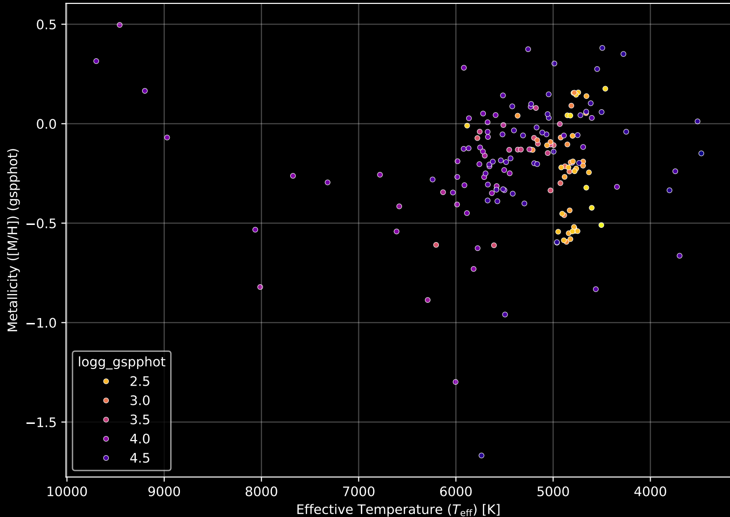
APOGEE DR17 Field: [223+27_MGA] Stellar Population Parameters (n= 167)
